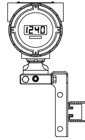
VERTICAL MOUNT TO HORIZONTAL CHANNEL
