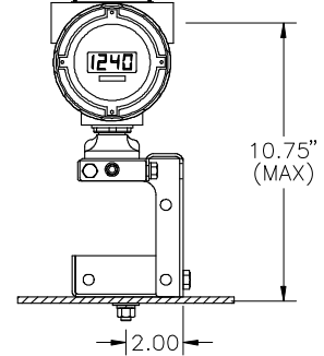
ANGLE MOUNT TO FLAT SURFACE
